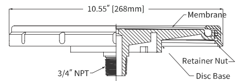
Disc Diffuser
