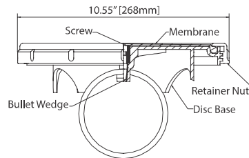
POD Connection
