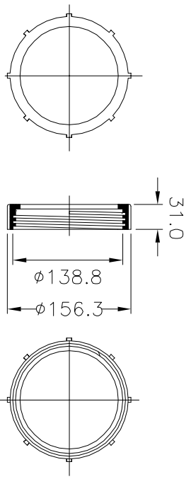
② Locknut
