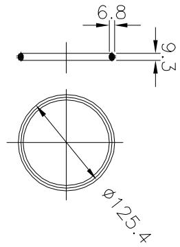
③ O-Ring
