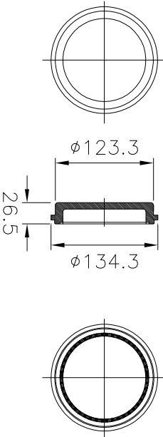
① End-Cap
