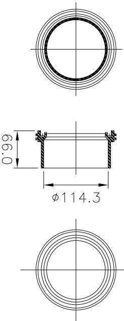
④ Male Housing
