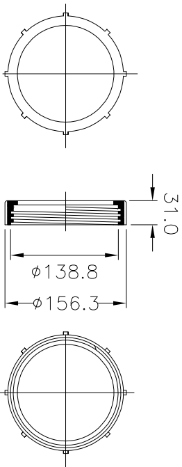
② Locknut
