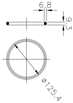
③ O-Ring
