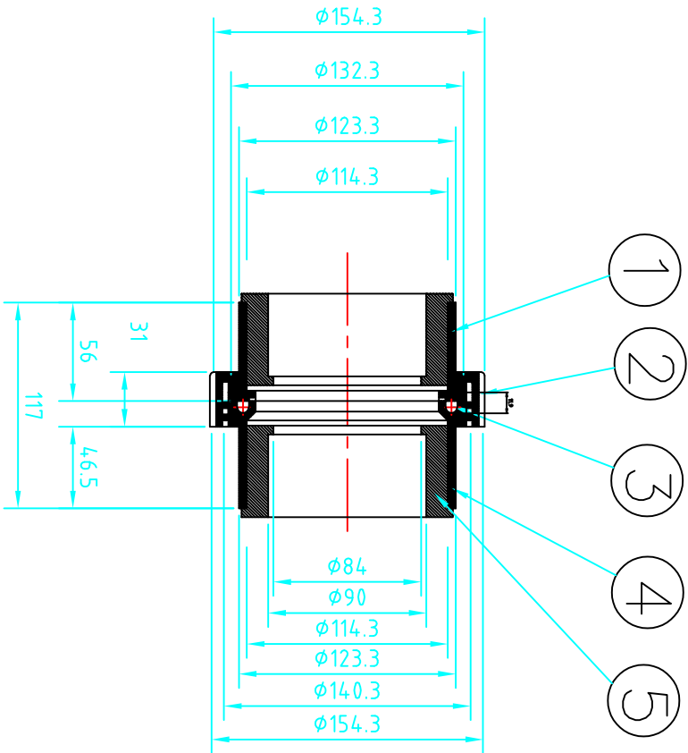
3" Adapter ASSEMBLY
