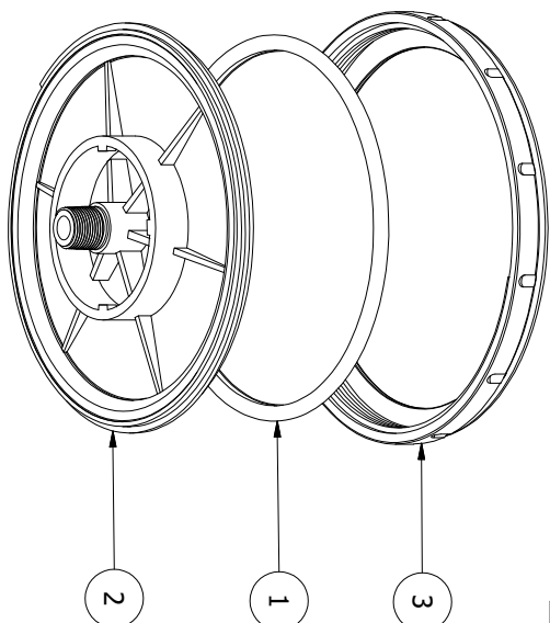
EXPLODED VIEW
