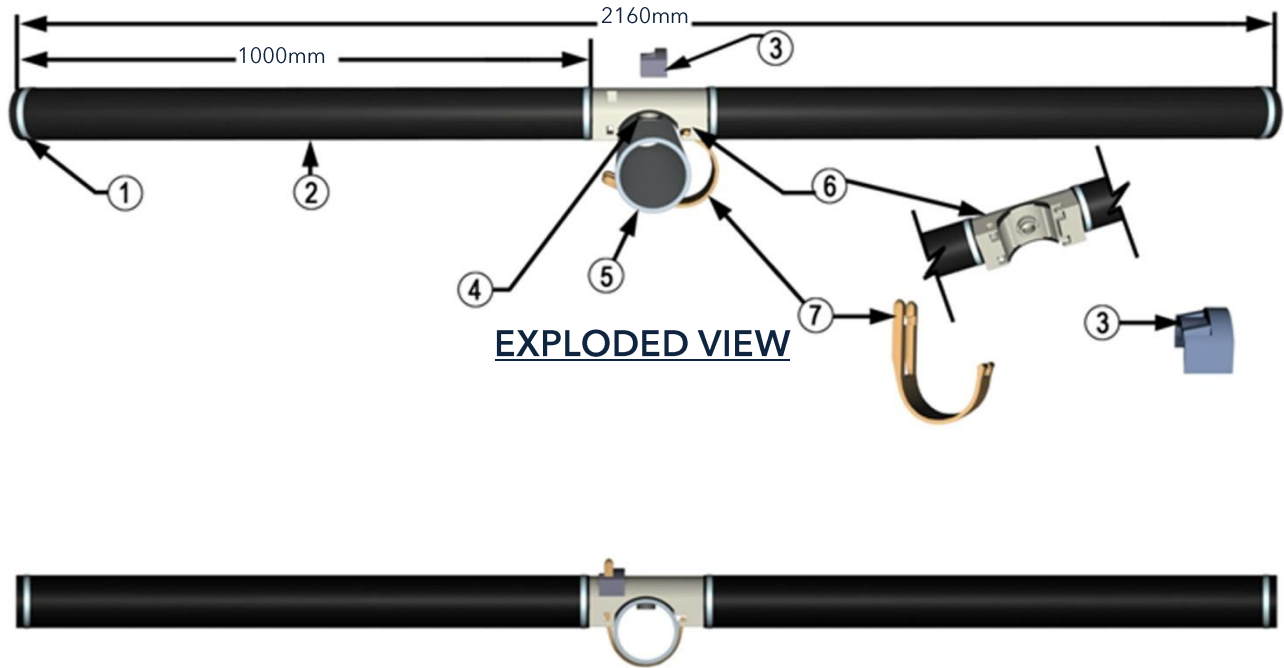
EXPLODED VIEW ASSEMBLED VIEW
