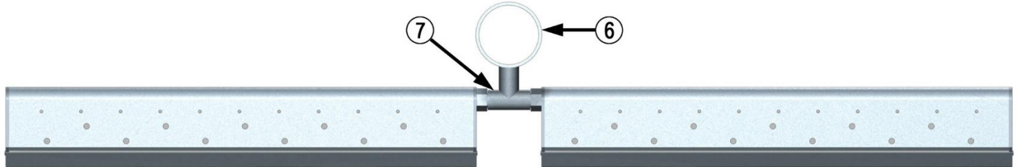
COARSE BAND DIFFUSER ASSEMBLED WITH Ø \frac{3}{4} " NPT (F) TEE
