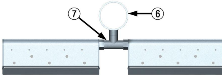
COARSE BAND DIFFUSER ASSEMBLED WITH Ø¾" NPT (F) TEE
