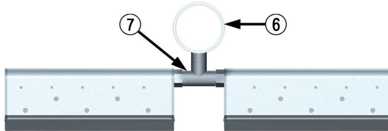
COARSE BAND DIFFUSER ASSEMBLED WITH Ø3/4" NPT (F) TEE
