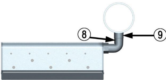
COARSE BAND DIFFUSER ASSEMBLED WITH Ø3/4" NPT (F) ELBOW
